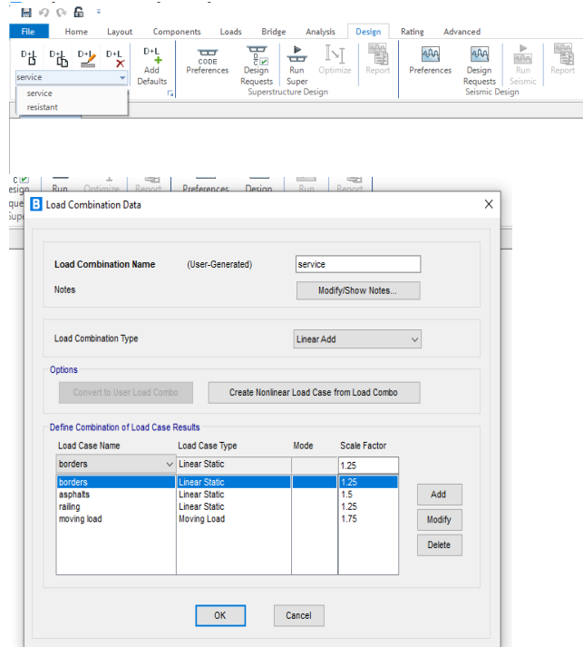
Fig-3 Load Combination Data
