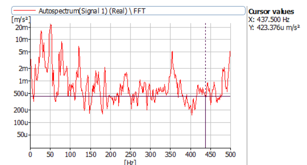
Fig-7 Truck wheeler reading
