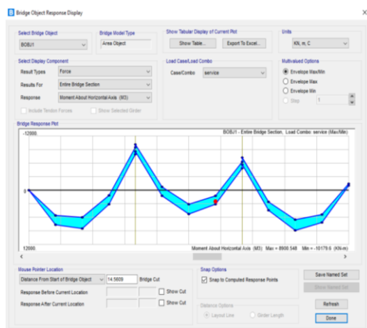
Fig-8 B.M. For load combination (service)
