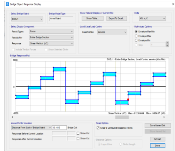
Fig-9 S.F. For load combination (service)
