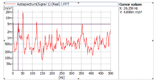
Fig-5 two wheeler reading
