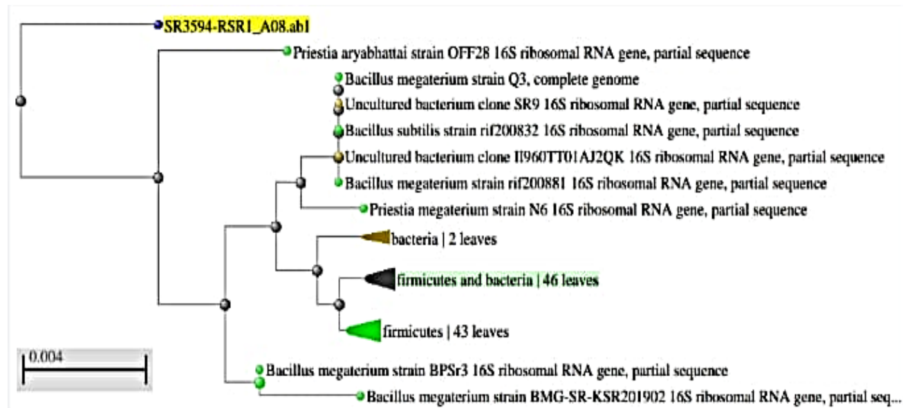
Fig 8: Phylogenetic Tree
