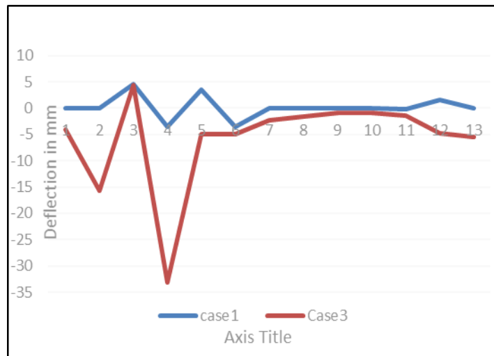
Fig 7: Structure Deflection comparison graph between case 1 and case 3
