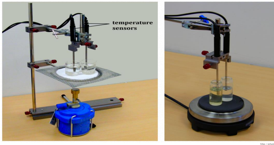
Fig-2: Experimental setup for radiation measurements for two different fluids
