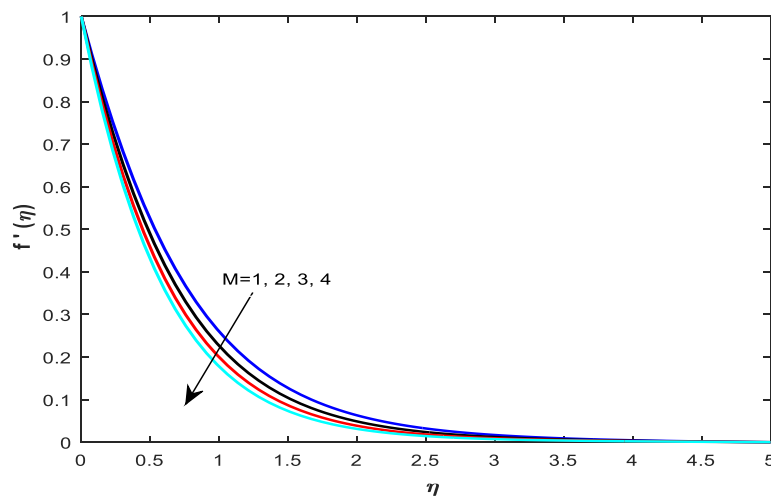
Fig 3. The effect of magnetic parameter M on the velocity profile
