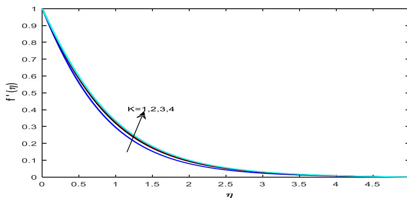
Fig 4. The effect of permeability parameter K on the velocity profile
