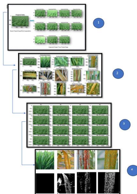
Figure 3: Data preprocessing
