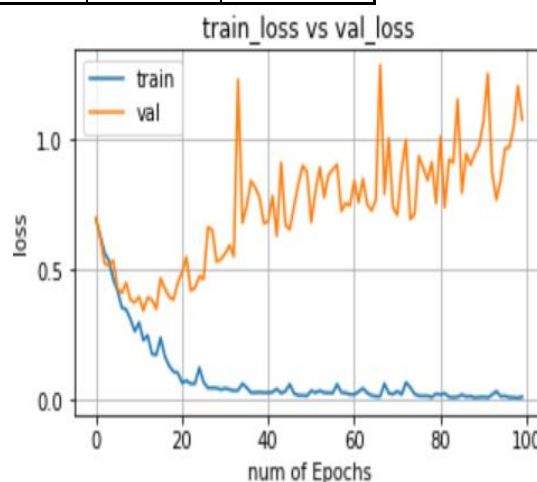
Figure 5: Training loss and validation loss comparison
