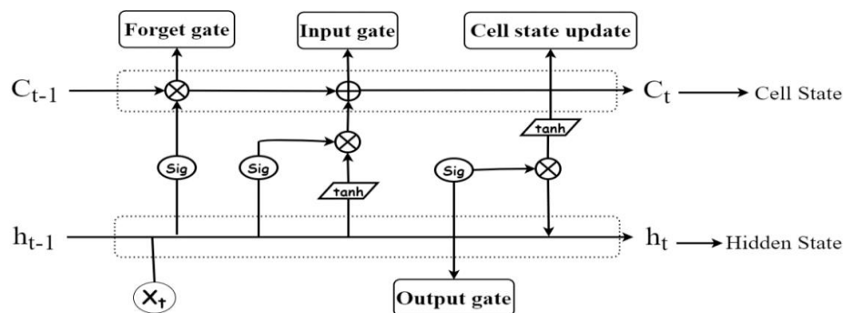
Fig. 1.LSTM Architecture
