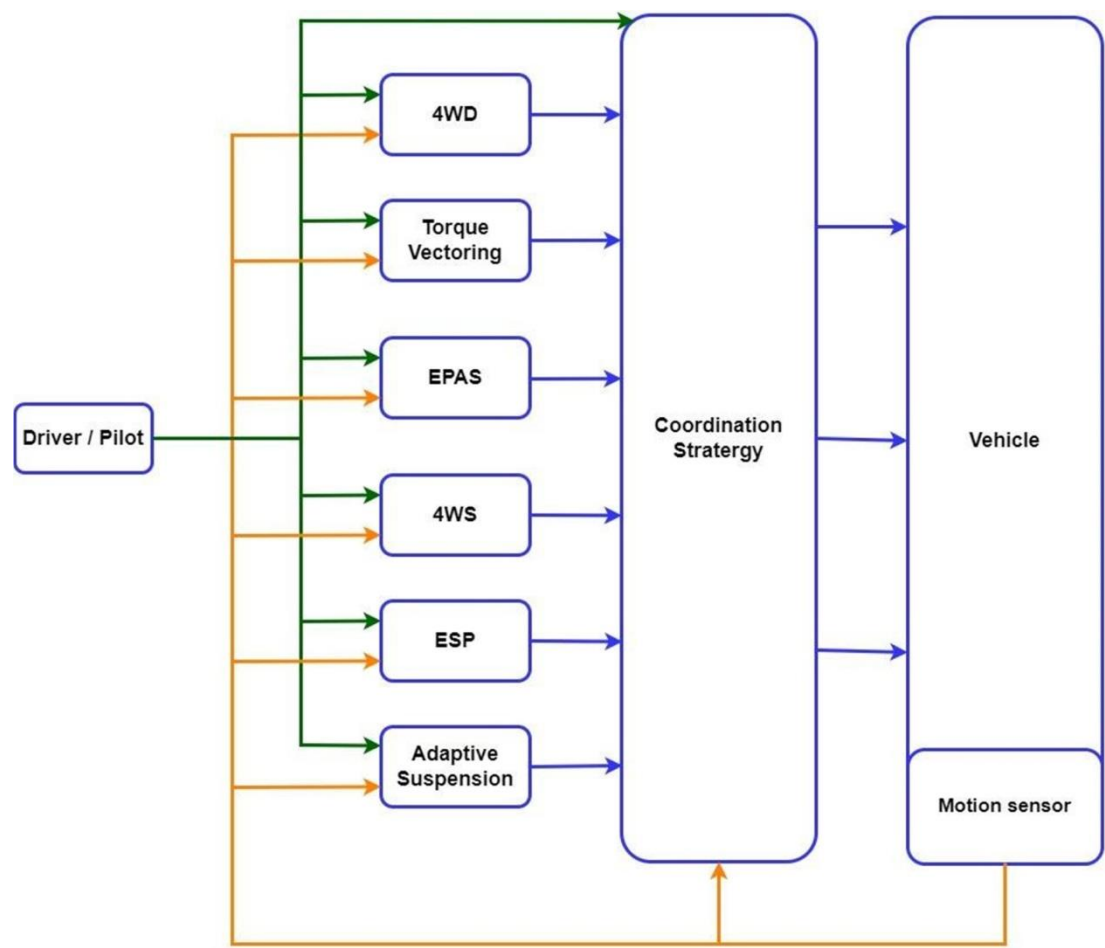
Figure. 1 Basic blocks of the downstream coordination system [10]
