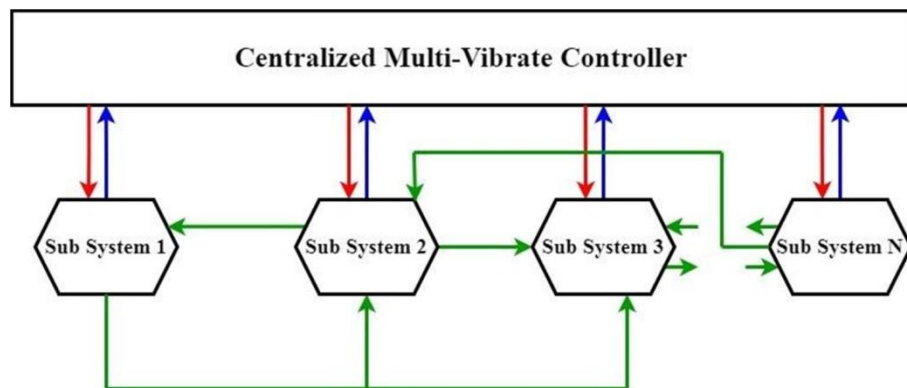
Figure. 4 Centralized-control architecture [10]
