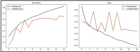
Fig. 7. ResNet50 Train/Test Plots
