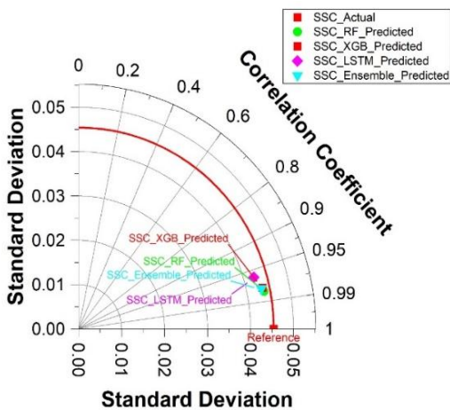
Figure 6. Taylor diagram for testing dataset showing comparative performance of RF, XGB, LSTM, and Stacked Ensemble models in predicting SSC.
