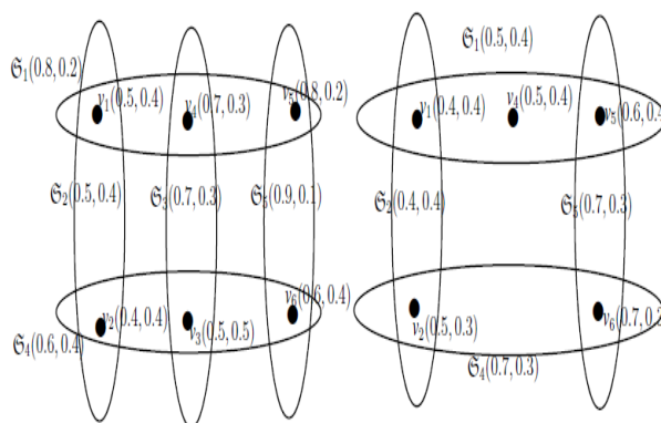
Figure 1: The IFSHG \tilde{H} = \{ \tilde{H}(a_1), \tilde{H}(a_2) \} corresponding to the parameters a_1 and a_2 .
